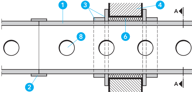
Detail F
